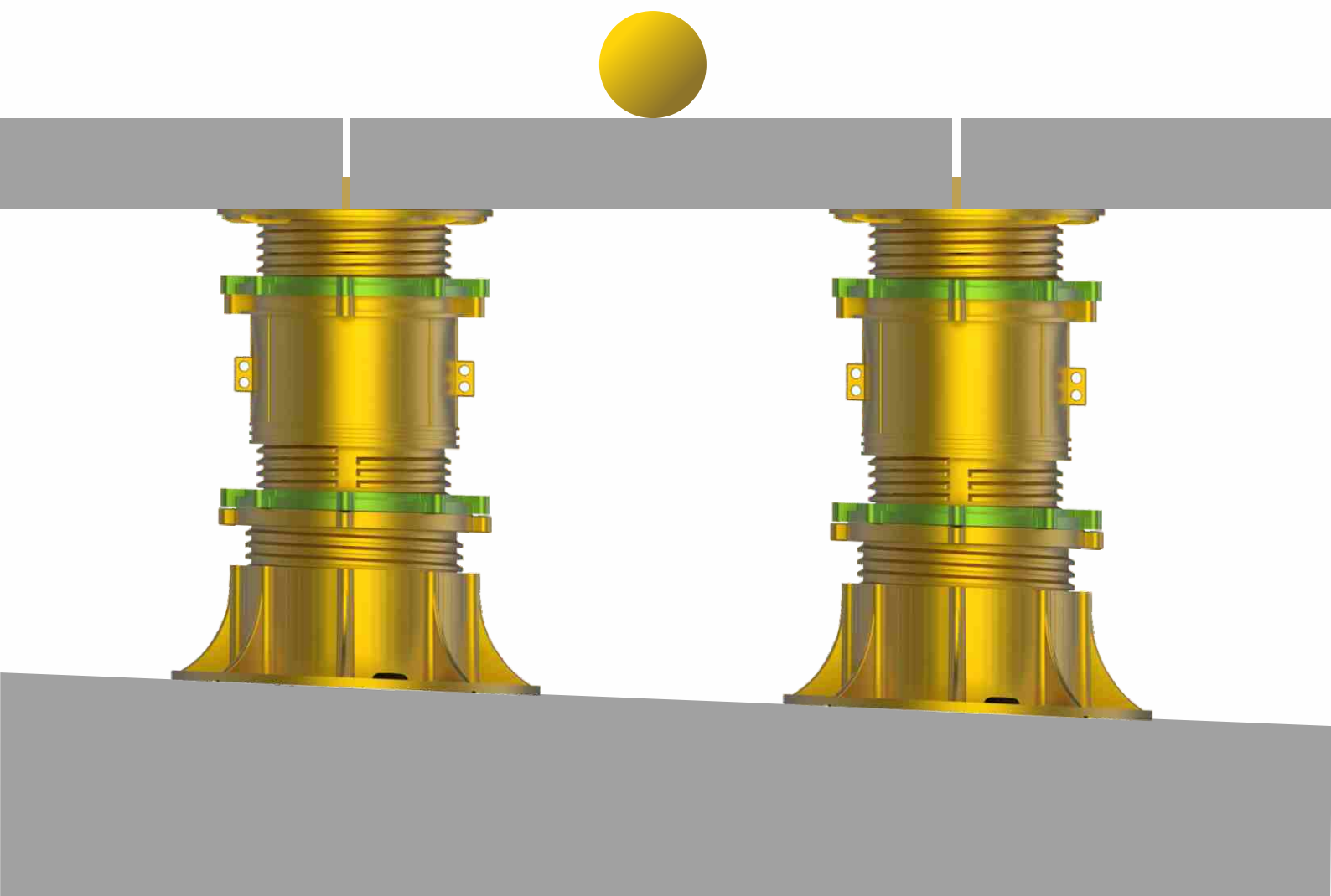
坡度调节 : 0-5% Slope compensation
